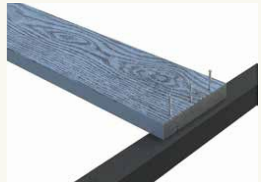
Three screws at board end
